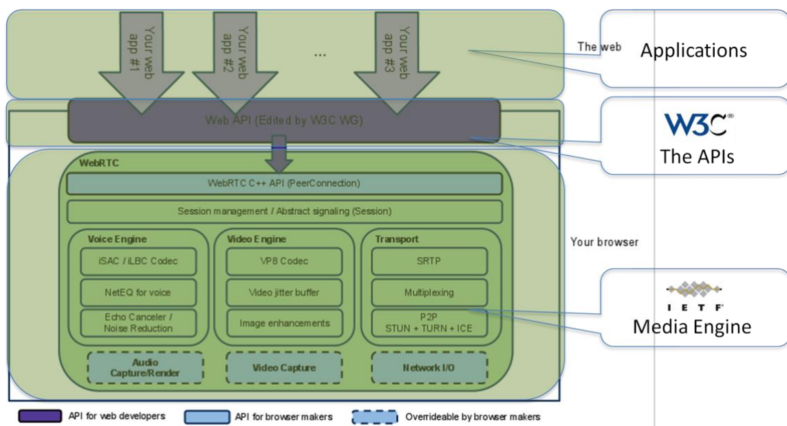
Figure 1 WebRTC framework
